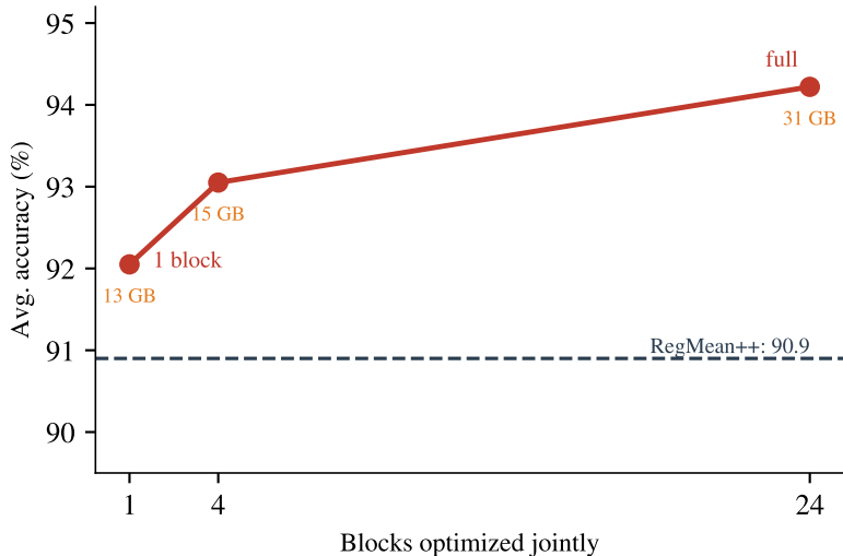
ViT-L/14 (24 blocks)
