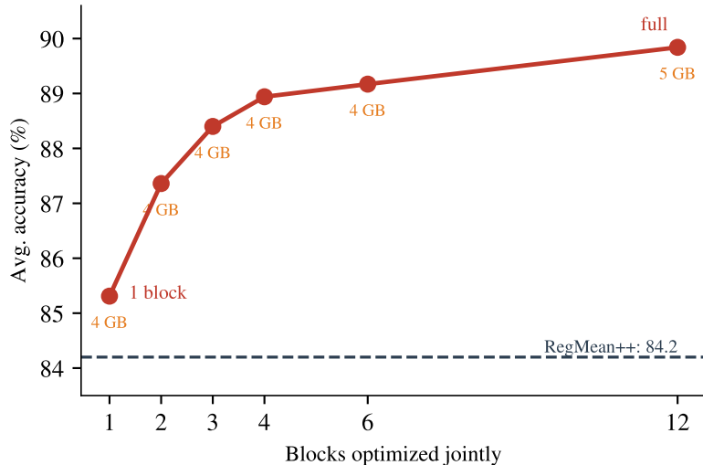
ViT-B/32 (12 blocks)
